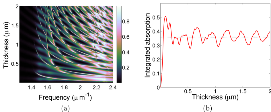
Figure 5. (a) Absorption as a function of frequency and photonic crystal slab thickness, for constant period \Lambda = 438 nm and hole radius r = 0.431\Lambda . (b) Integrated absorption as a function of photonic crystal slab thickness.
