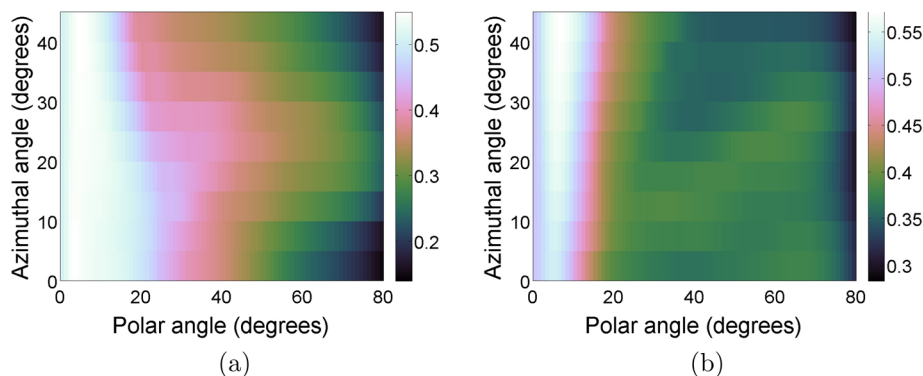
Figure 6. Frequency-integrated absorption as a function of angle for (a) p-polarization and (b) s-polarization.
