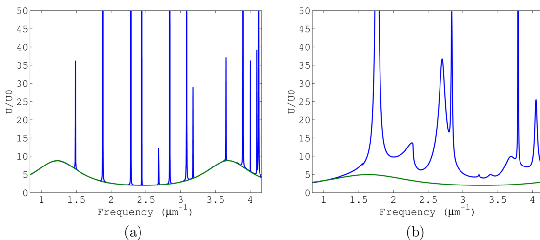
Figure 2. Energy density enhancement for a photonic crystal slab backed by a PEC mirror (blue curves), compared to that in an unpatterned dielectric slab on a PEC mirror (green curves). (a) The photonic crystal slab has \Lambda = 438 nm, r = 0.043\Lambda , d = 97 nm, n = 2.1 . The homogeneous dielectric slab has d = 97 nm, n = 2.1 . The high-Q guided resonances are superimposed on top of a Fabry–Perot background. (b) The photonic crystal slab has the same period and thickness, but r = 0.43\Lambda , while the homogeneous dielectric slab has d = 97 nm and n = 1.6 .
